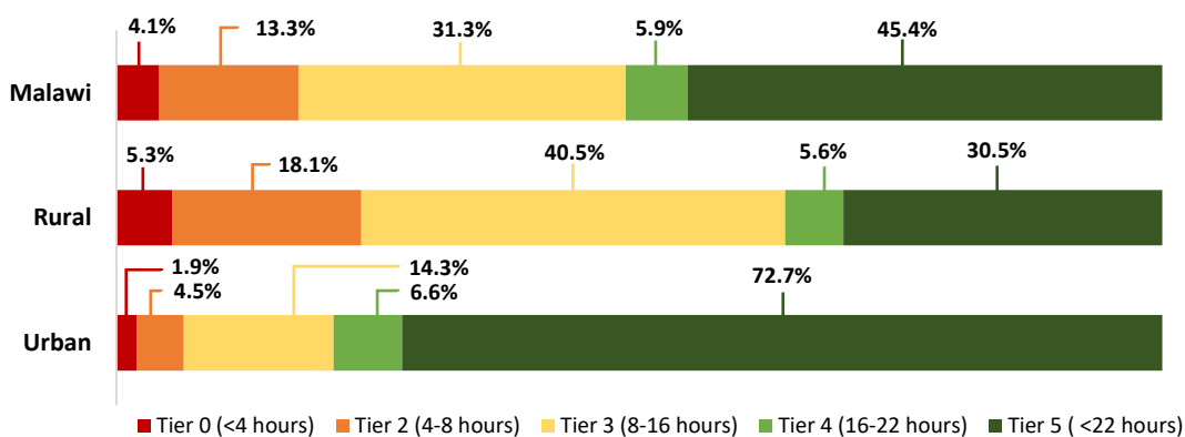
Figure 18 : Share of households with daily access to electricity by place of residence
