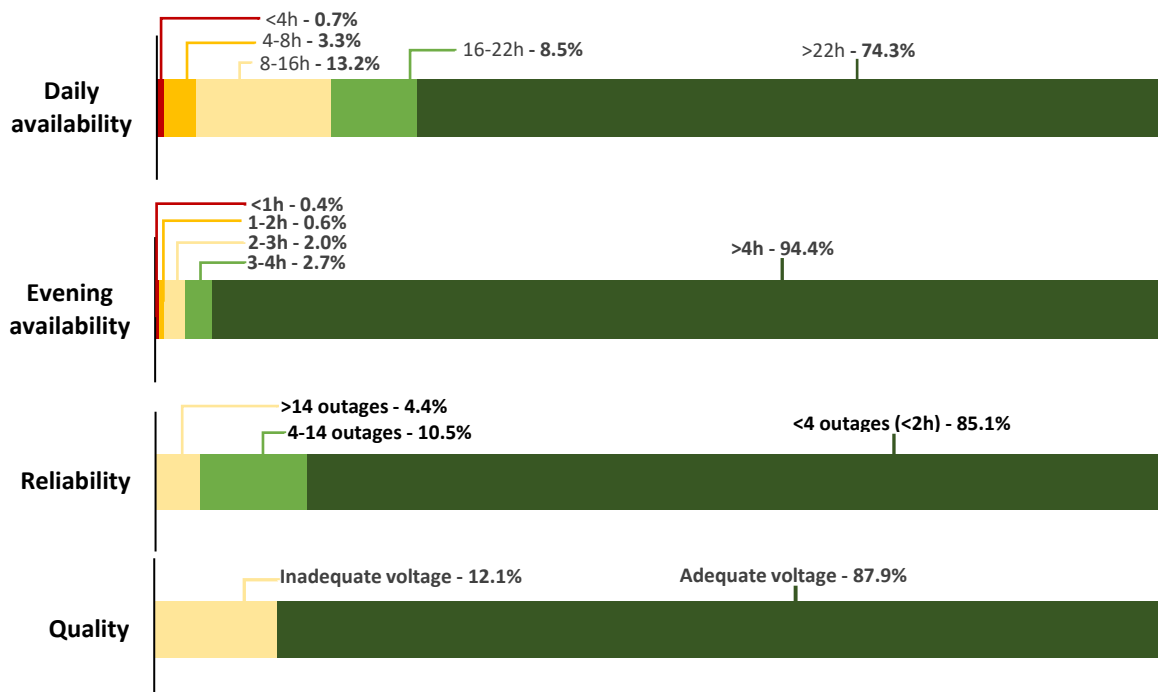
Figure 41: Distribution of grid-connected households by Multi-Tier Framework attributes
